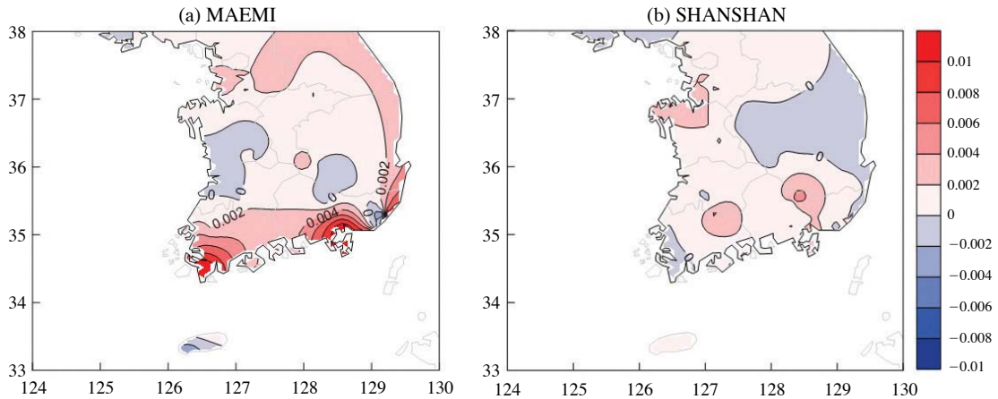
Fig. 7. The increased cases of \text{SO}_2 concentration for \Delta C_2 .
