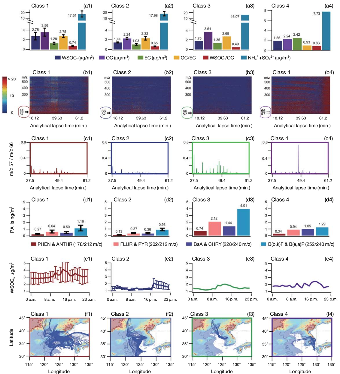
Fig. 5. (a) WSOC i , OC, EC, OC/EC, WSOC i /OC, and sum of SO 4 2- and NH 4 + related to classes, (b) total ion mass (m/z) distributions by GC/MS-TD related to classes, (c) m/z 57 / m/z 66 by GC/MS-TD related to classes, (d) PAHs by GC/MS-TD related to classes, (e) diurnal patterns of WSOC p related to classes, (f) back trajectories related to classes.
