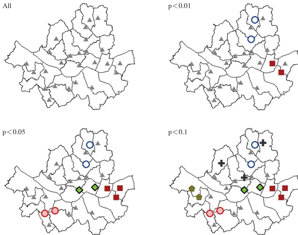
Fig. 1. Grouping of air monitoring stations by cluster analysis using daily highest 8-hour ozone concentrations plus corresponding 8-hour \text{NO}_2 concentrations. P-value indicates how strong the cluster is supported by data; the smaller the p-value, the larger the significance of clusters. Symbols in the 'all' panel denote all monitoring stations in Seoul. Different symbols denote different clusters of stations.
