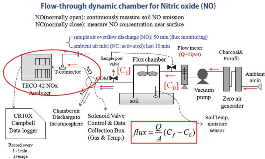
Fig. 1. A schematic flow-through dynamic chamber system for surface NO emission in x-y plot during August 13~15, 2013.
