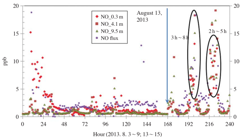
Fig. 2. Ambient NO concentrations for three different heights, and surface NO soil emission ( \mu g m^{-2} hr^{-1} ) measured by FDC method.
