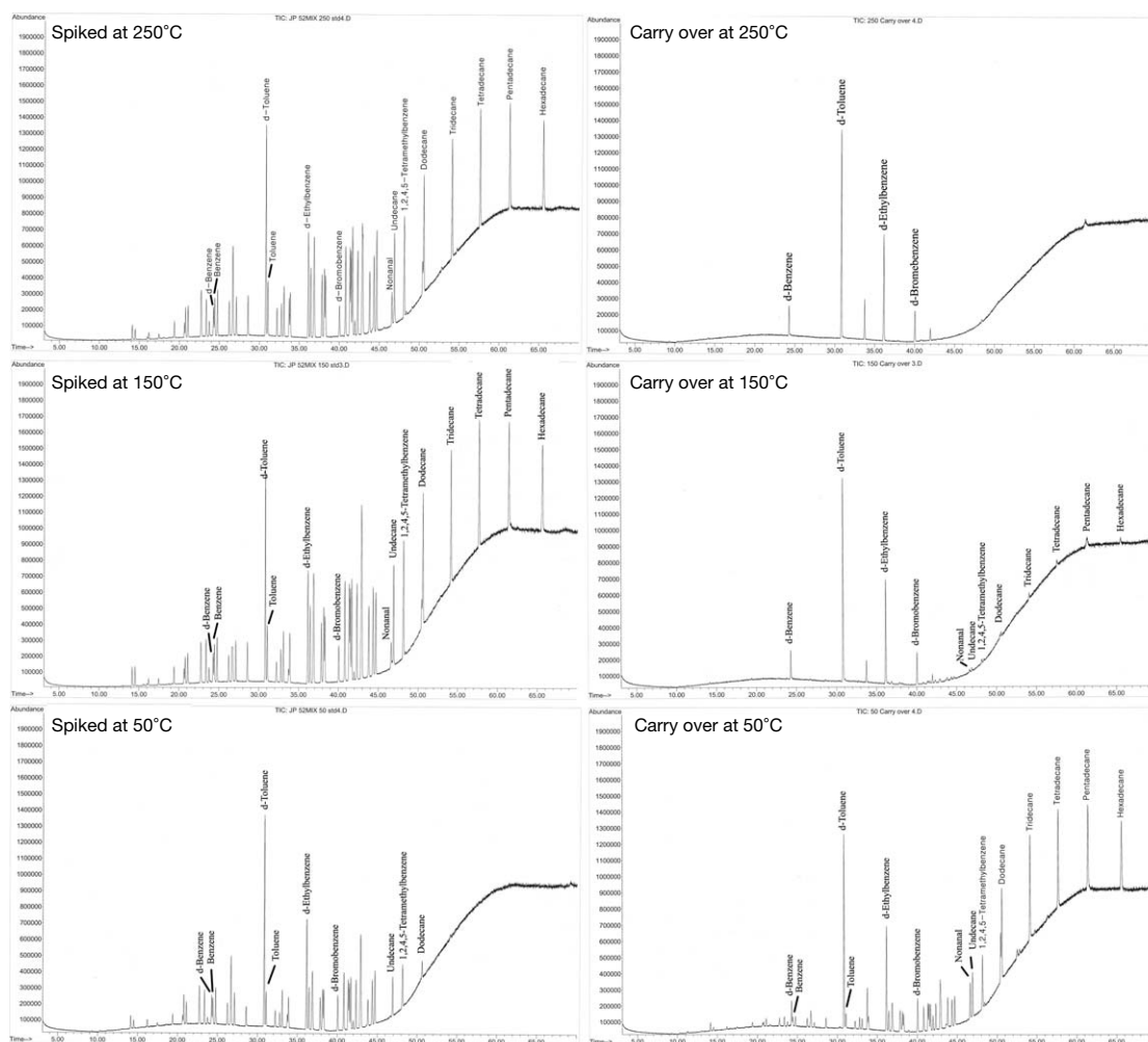
Fig. 4. Each temperature impregnation GC/MSD chromatogram.
