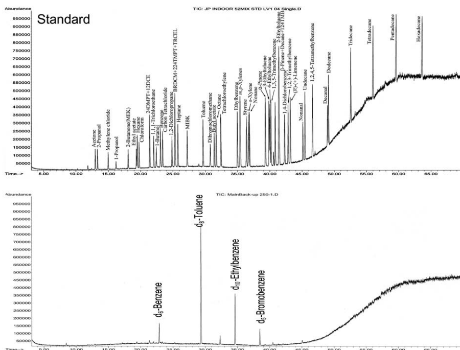
Fig. 2. Typical GC/MS chromatograms for a 52 mixture of liquid standards (top) and internal standards (bottom).
