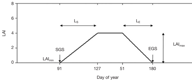
Fig. 2. Schematic of LAI development and associated parameters. SGS and EGS are the start and end of the growing season, in day-numbers. L_s and L_e represent the length of the LAI-increase and decline periods, also in-day numbers. Maximum and minimum (within the growing season) LAI values are given by LAI_{max} , LAI_{min} , respectively.
