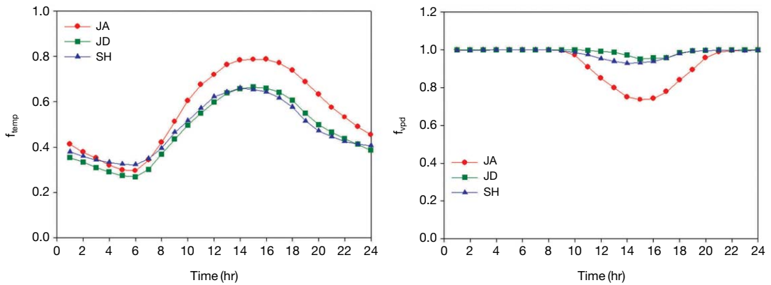
Fig. 6. Diurnal variation of the parameters f_{\text{temp}} and f_{\text{vpd}} at 3 sites (April 1 ~ June 30, 2006).
