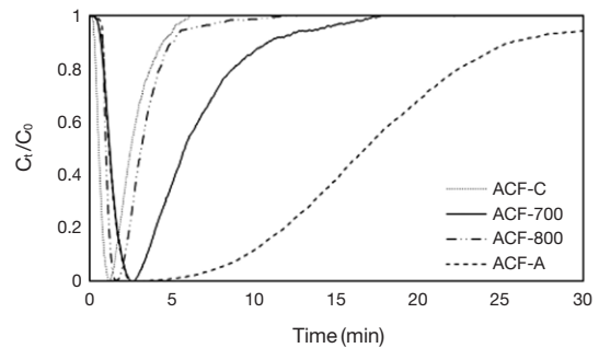
Fig. 6. Breakthrough adsorption curves for 0.3% CO 2 flow.
