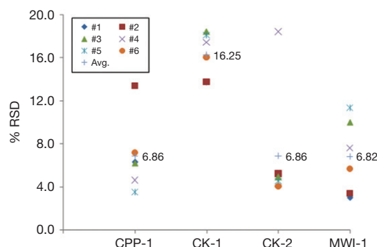
Fig. 6. % RSD between EPA Method 101A and EPA Method 30B.
