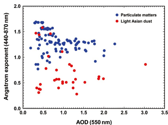
Fig. 3. Distribution of Ångström exponent and AOD retrieved from GOCI for high particulate matters (blue) and light Asian dust (red) cases.
