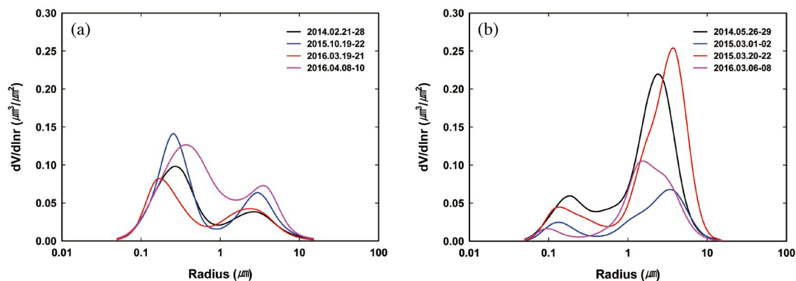
Fig. 4. Comparison of volume size distributions for (a) high particulate matters and (b) light Asian dust.
