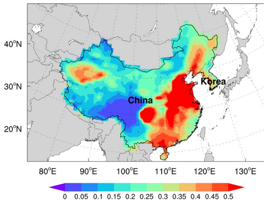
Fig. 2. Study area and spatial distribution of MODIS-AOD averaged over 20 years (from Feb. 2001 to Dec. 2020) in East Asia.
