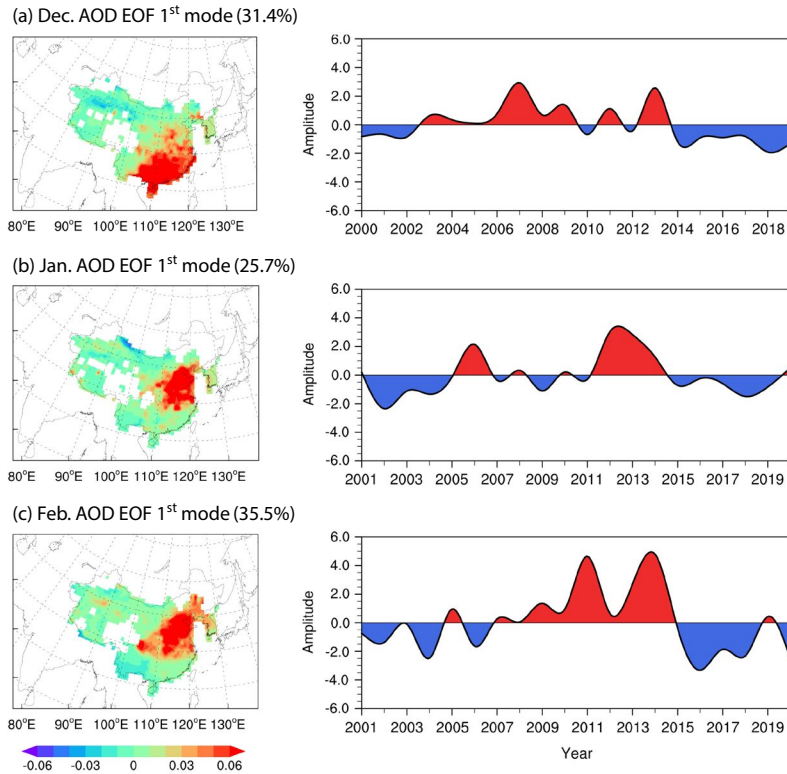
Fig. 4. The 1 st principle components of wintertime (Dec., Jan., and Feb.) aerosol optical depth (AOD PC1), and their time series for three month: (a) December, (b) January, and (c) February, during 2000~2020.
